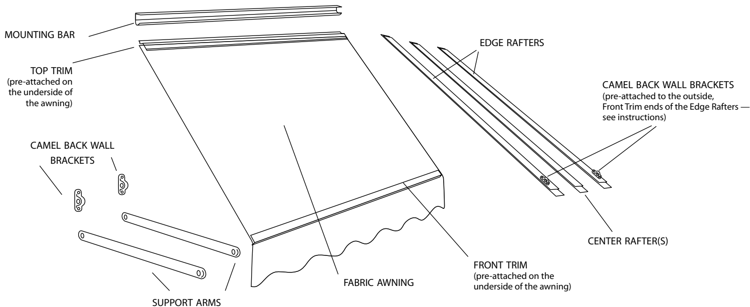
Series 3300 with Support Arms
